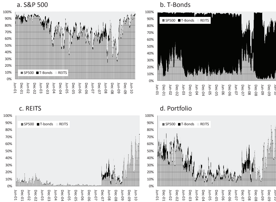
Figure 2: Variance decompositions
