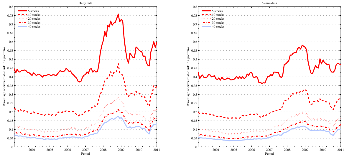
Figure 5: DIVERSIFIABLE RISK REMAINING FOR PORTFOLIOS OF VARIOUS SIZES. As the number of stocks in portfolios increases the percentage of diversifiable risk remaining changes over the years. The panels above show the dynamics of diversifiable risk remaining for portfolios of various sizes. Results are obtained for an investor seeking to diversify with assurance 90% of the time. The left panel is based on standard deviations with daily data; the panel on the right uses 5-minute data and is based on the realized volatility.
